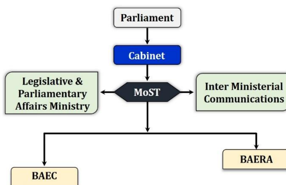
Figure 2. Structure of Bangladesh government related to nuclear energy and radiological affairs.
